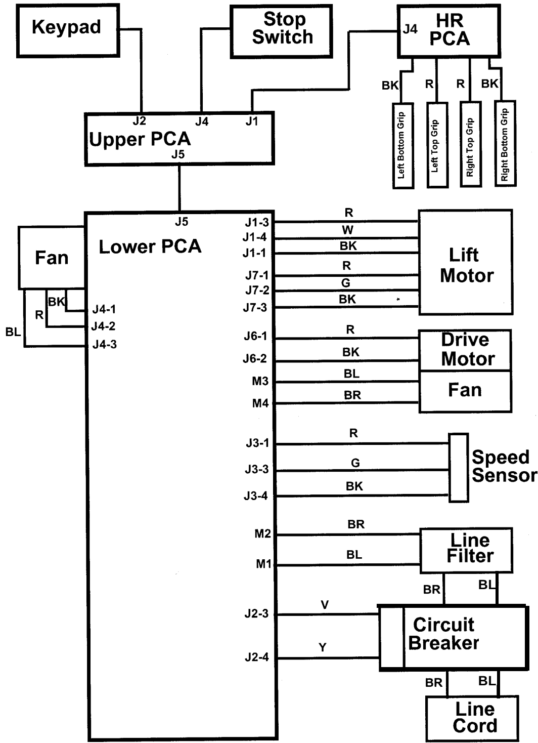
Wiring Diagram 7.2 — C966-240 Vac
